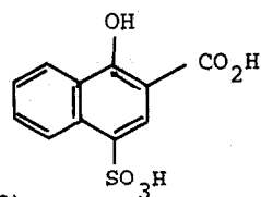
1-hydroxy-4-sulphonato- 2-naphthoic acid.
