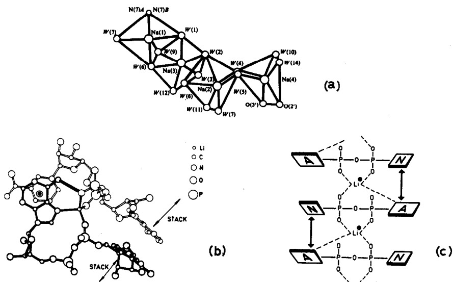
Figure 10. Coordination polyhedra of (a) \text{Na}^+ in [\text{GMP}]\text{Na}_2\cdot\text{H}_2\text{O} and (b) \text{Li}^+ in \text{Li}^+\cdot\text{NAD}^+\cdot 2\text{H}_2\text{O} . Schematic diagram (c) of the stacking in \text{Li}^+\cdot\text{NAD}^+\cdot 2\text{H}_2\text{O} (reproduced by permission from (a) Acta Crystallogr. , B37(1981)1825 and (b,c) J. Am. Chem. Soc. , 103(1981)907).
