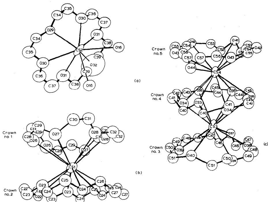
Figure 6. Ortep diagrams of the fragments of the [(18C6)_{14}Cs_9]^{9+} cationic complex of [(18C6)_{14}Cs_9]^{9+}[Rh_{22}(CO)_{35}H_x]^{5-} , [R_{22}(CO)_{35}H_{x+1}]^{4-} : (a) [(18C6)Cs]^{+} , (b) [(18C6)_2Cs]^{+} , (c) [(18C6)_3Cs_2]^{2+} (reproduced by permission from Inorg. Chem., 20(1981)227).
