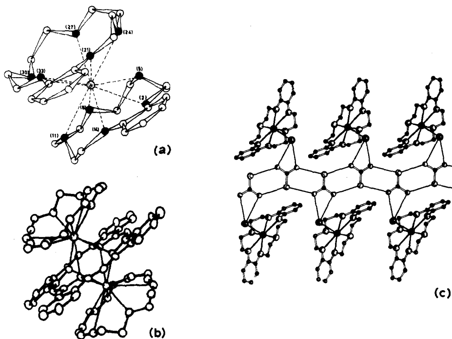
Figure 4. Perspective views of the K^+ coordination sphere in (a) (B15C5)_2 \cdot K[picrate] , (b) (18C6)_2 \cdot K_2[phthalocyanine] and (c) DB18C6 \cdot KI \cdot (NH_2)_2CS (reproduced by permission from (a) Inorg. Nucl. Chem. Letters , 17(1981)207, (b) J. Am. Chem. Soc. , 103(1981)4629 and (c) Angew. Chem. Int. Ed. Engl. , 20(1981)1045).
